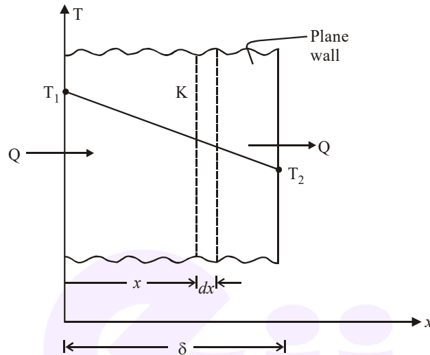
Temperature profile (PLANE . WALL)
