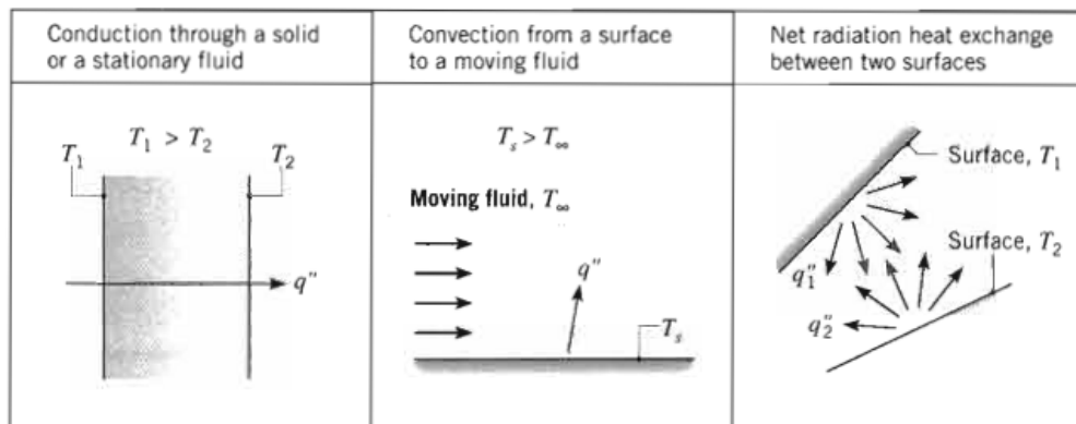
Figure – 1: conduction, convection and radiation heat transfer modes.
