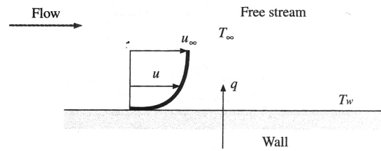
Figure-2: convection heat transfer from a plate.
