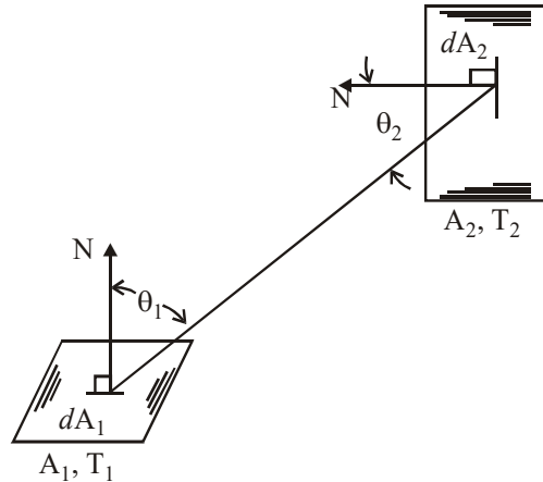
Figure: Radiant Heat exchange
